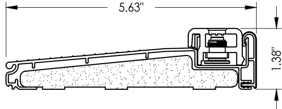
5 INSWING THRESHOLD
