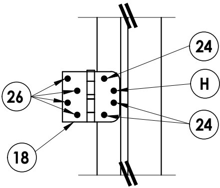
HINGE DETAIL
