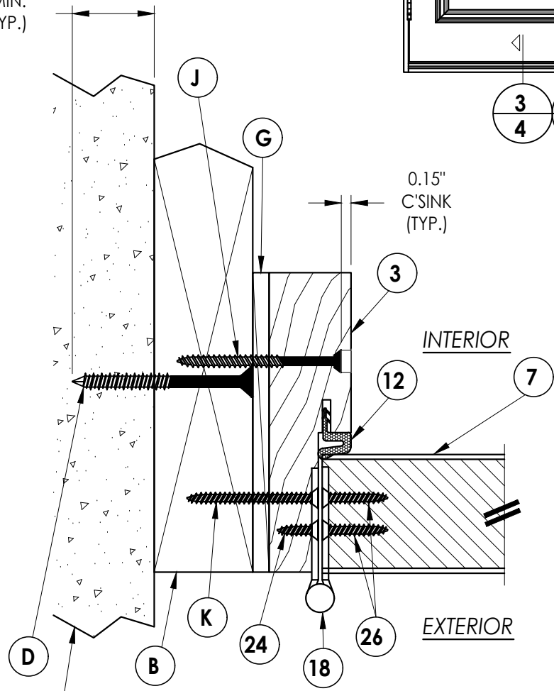
1 3 HORIZONTAL CROSS SECTION Outswing shown - inswing also approved
