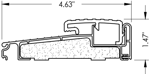
25 OUTSWING THRESHOLD Low profile ADA
