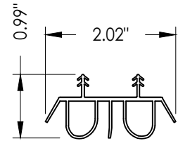
6 SWEEP
