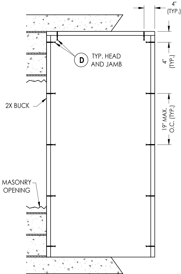
BUCK ANCHORING
